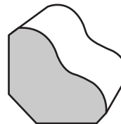
F660 9/16" x 1-1/8"
