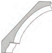
F641 1-1/16" x 7-1/4"
