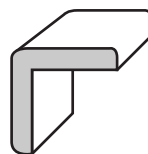
OUTSIDE CORNER 204 1-5/16" 205 1-1/8" 206 3/4"
